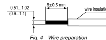
Fig. 4 Wire preparation
