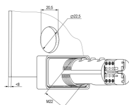
Fig. 2 Mounting cutout
