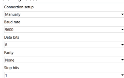
Fig. 14 Connection setup
