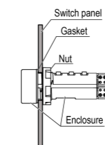
Fig. 1 Mounting
