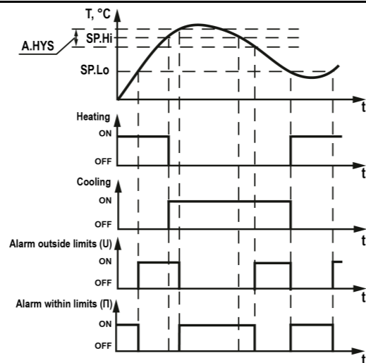
Fig. 10 Output device logic
